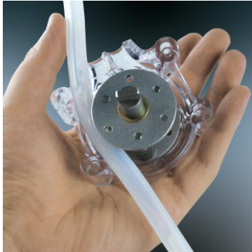
1. Disassemble the pump head, and press the tubing on the rollers.
